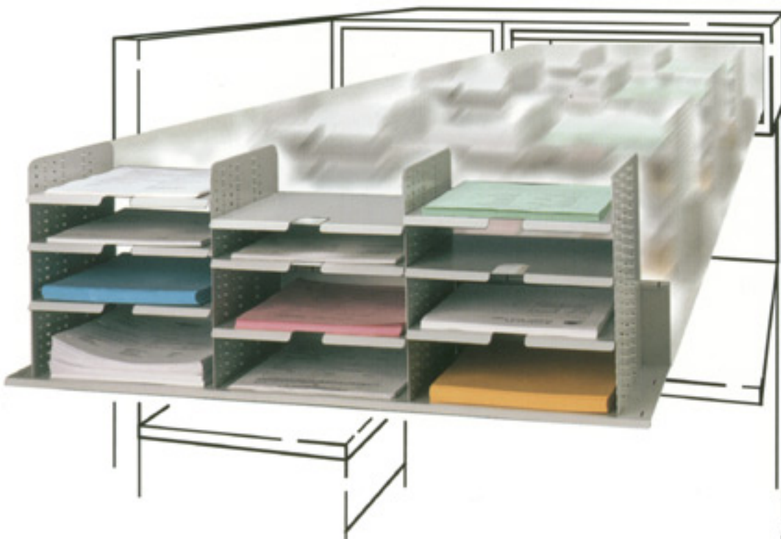
Manager's System, KB3312D, 33"W x 12"D x 11 3/4"H with 12 pockets, each 10"W x 12"D x 3"H.
